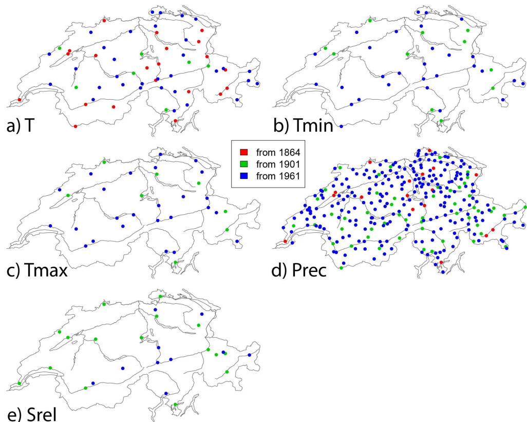
Figure 2. Location of stations with continuous and homogeneity-tested data series since 1864 (red), 1901 (green and red) and 1961 (blue, green and red) for mean temperature, mean minimum temperature, mean maximum temperature and precipitation.
